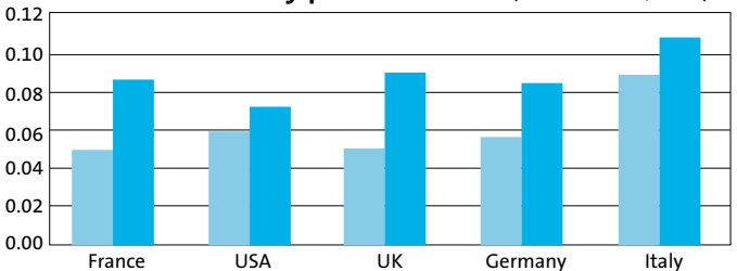
Industrial electricity prices increases (2001-2006 €/kWh)
